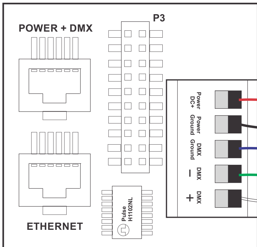
STICK-DE3 Back View Connectors Close-Up
